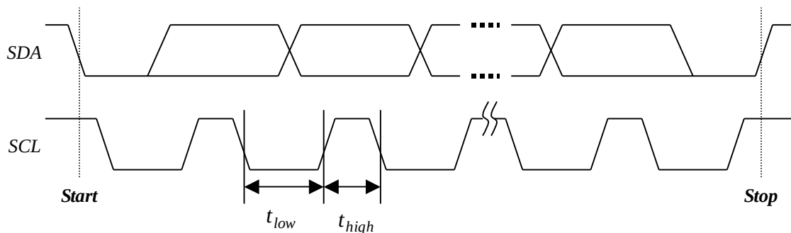
Fig. 7.5.6.1 Standard mode and fast mode timing.
